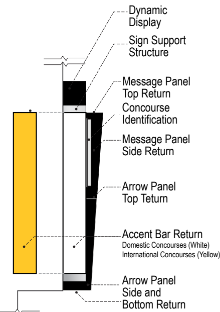
4 SIGN FINISHES - END VIEW SCALE: NTS
