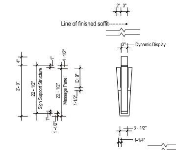
4 SIDE VIEW SCALE: 1/2" = 1' - 0"
