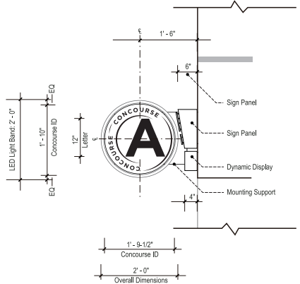
3 SIDE VIEW SCALE: 1/2" = 1' - 0"
