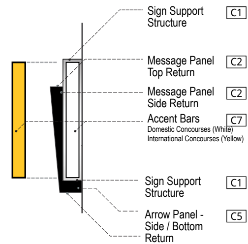
4 SIDE FINISHES - END VIEW SCALE: 1-1/2" = 1' - 0"
