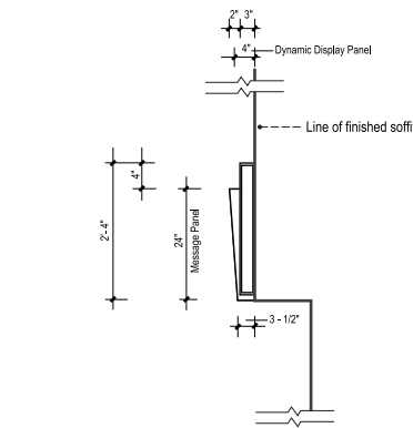
3 SIDE VIEW - SOFFIT MOUNT SCALE: 1/2" = 1' - 0"
