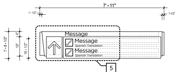
2 FRONT VIEW SCALE: 1/2" = 1' - 0"
