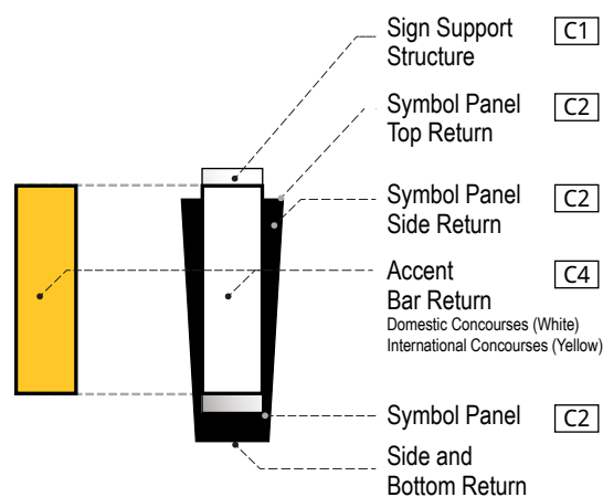
4 SIGN FINISHES - END VIEW SCALE: NTS
