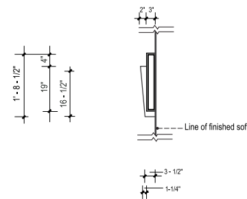
3 SIDE VIEW SCALE: 1/2" = 1' - 0"
