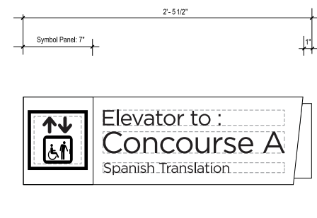
4 FRONT VIEW (ALT. LAYOUT) SCALE: 1 - 1/2" = 1' - 0"
