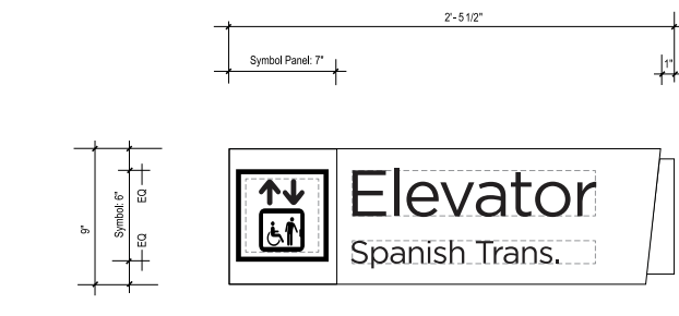
2 FRONT VIEW SCALE: 1 - 1/2" = 1' - 0"
