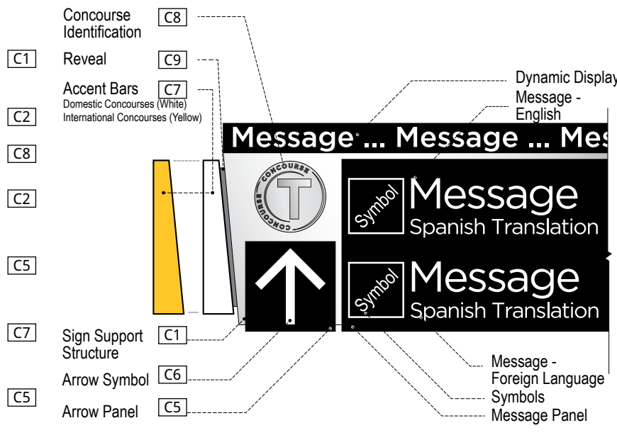
6 SIGN FINISHES SCALE: NTS
