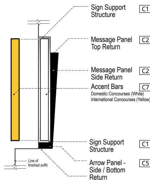
4 SIGN FINISHES - END VIEW SCALE: 1-1/2" = 1' - 0"
